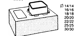
10 Modular flue (rear ventilated) with ventilation duct
